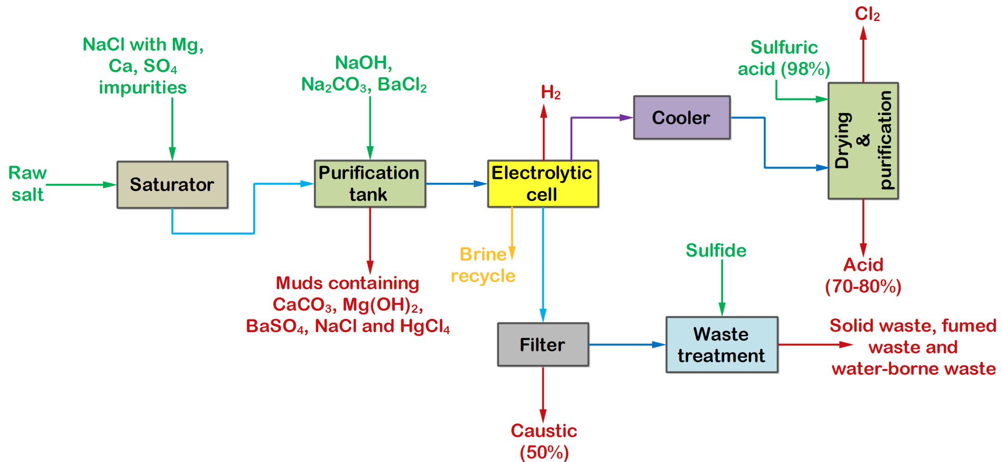
Figure: Manufacture of chlorine by mercury cell process
